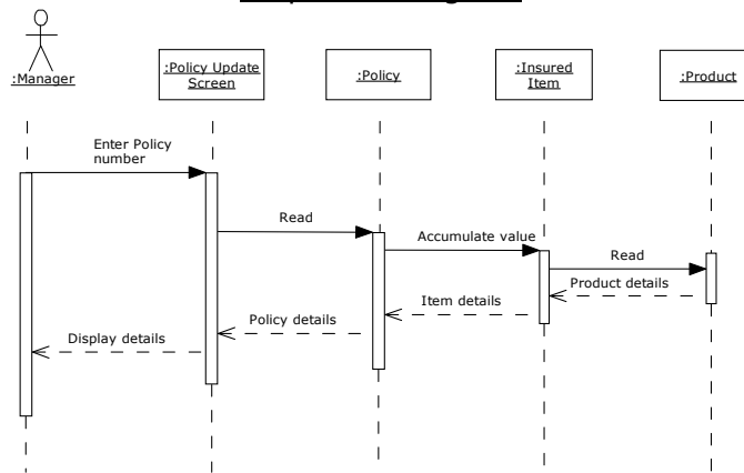
Sequence Diagram
